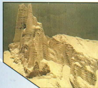
View of soya build up from down inside silo just prior to activation of one Cardox Tube.
